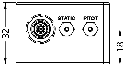
Illustration 1: Mechanical drawings of Air Data Unit
