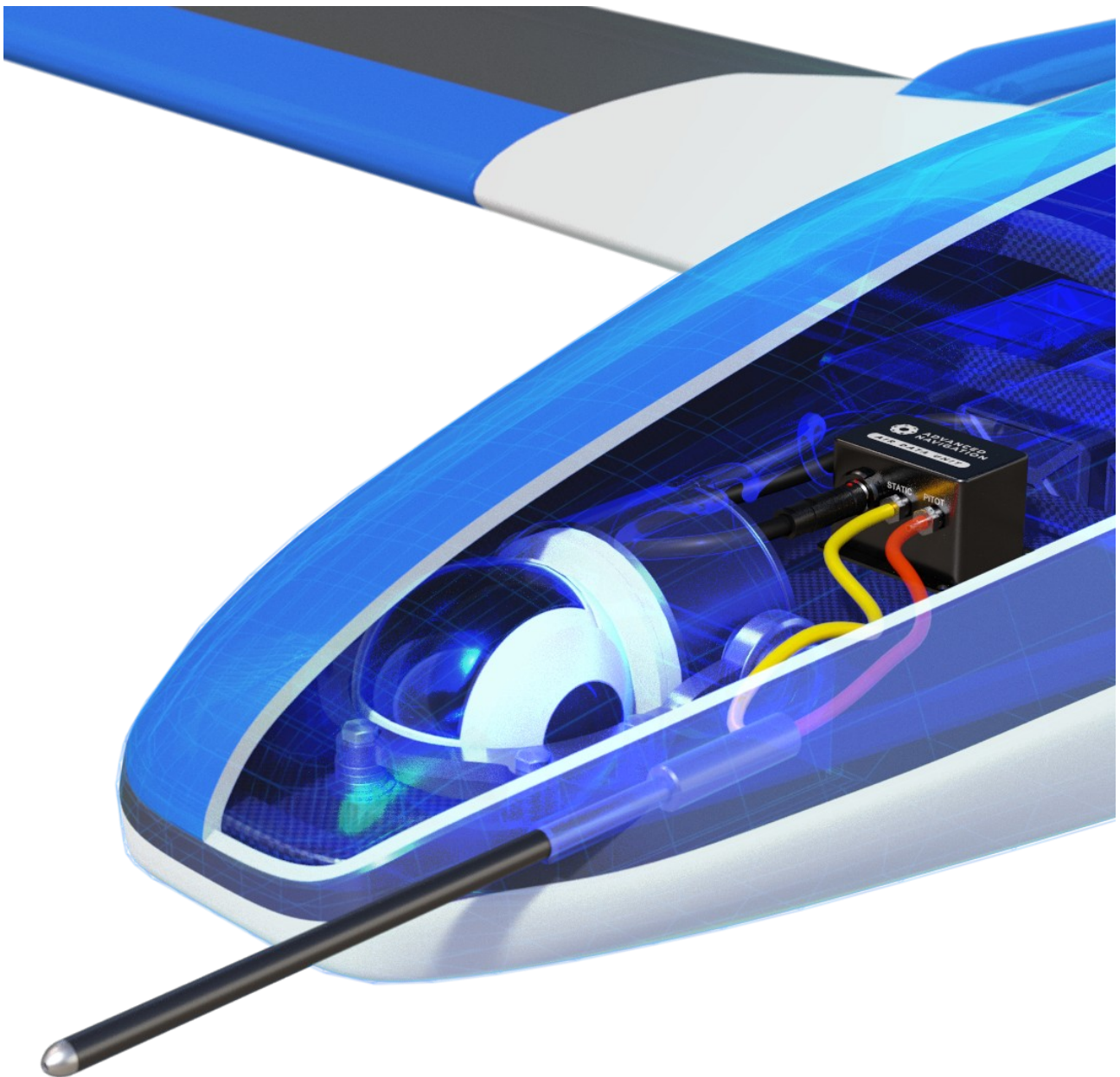
Illustration 6: Example air data unit installation
