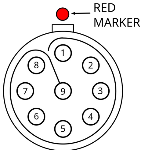
Illustration 3: ODU B series pin locations
